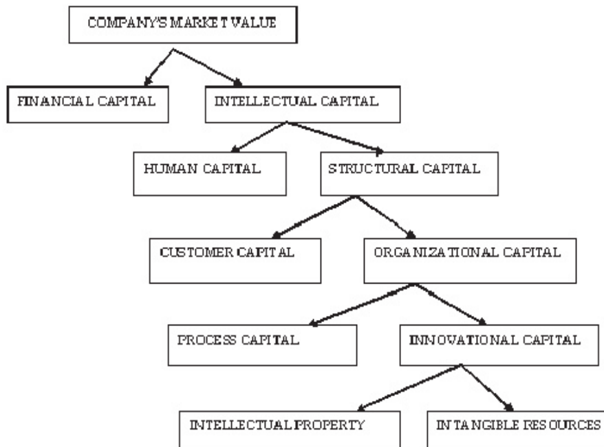
Figure 2. Skandia Model [8]
